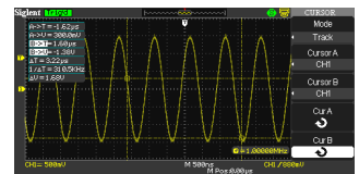
Cursor-measurement
