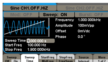
Sweep
