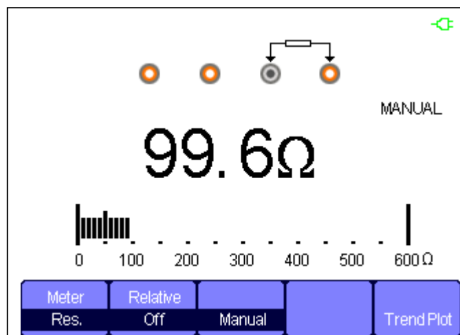
Figure 3-4 Resistance Measurement
