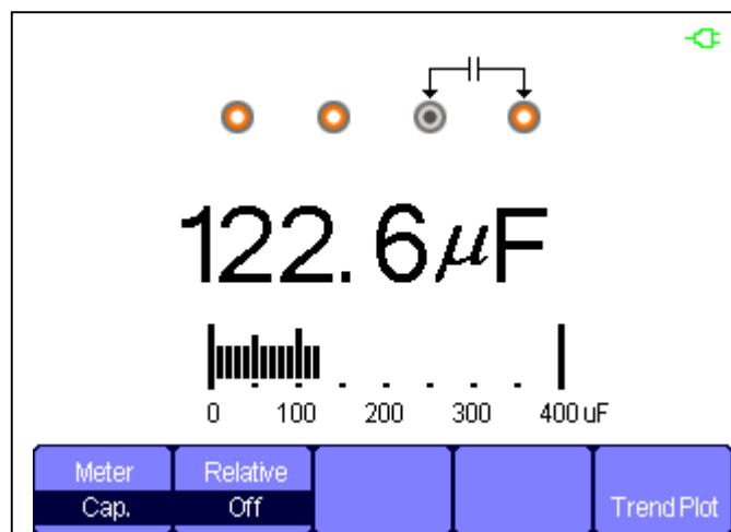
Figure 3-7 Capacitance Measurement
