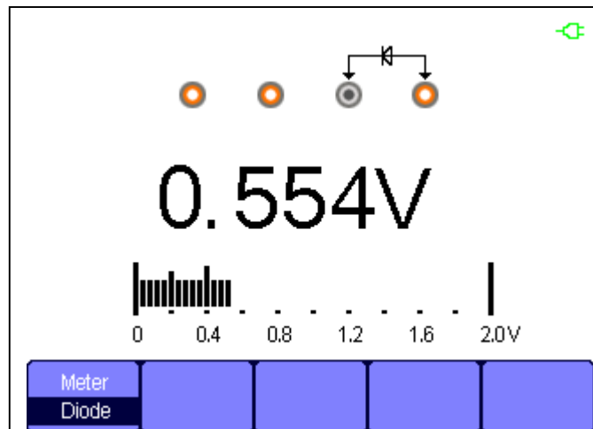
Figure 3-5 Diode Measurement
