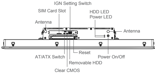
Front I/O
