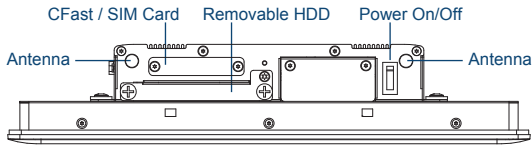
Front I/O
