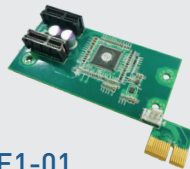
RC-E1E1-01 Riser Card with 2x PCIe1 Slots Interface: 1x PCIe1 Expansion: 2x PCIe1 Dimension: 111.3 x 60.5 mm
