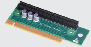
RC-E16-01 Riser Card with 1x PCIe16 Slot Interface: 1x PCIe16 Expansion: 1x PCIe16 Dimension: 111.3 x 40.5 mm
