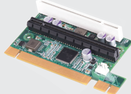
RC-E16PI-01 Riser Card with 1x PCIe16 and 1x PCI Slots Interface: 1x PCIe16 + 1x PCIe1 Expansion: 1x PCIe16, 1x PCI Dimension: 111.3 x 60.5 mm
