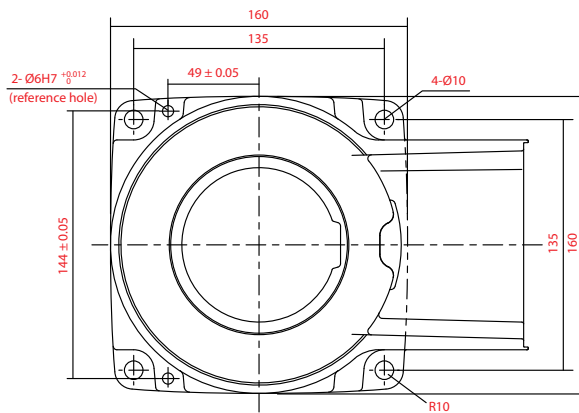
Detail of base mounting face (top view)
