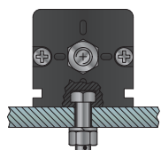
mounting with M5 screw ISO4017-DIN933
