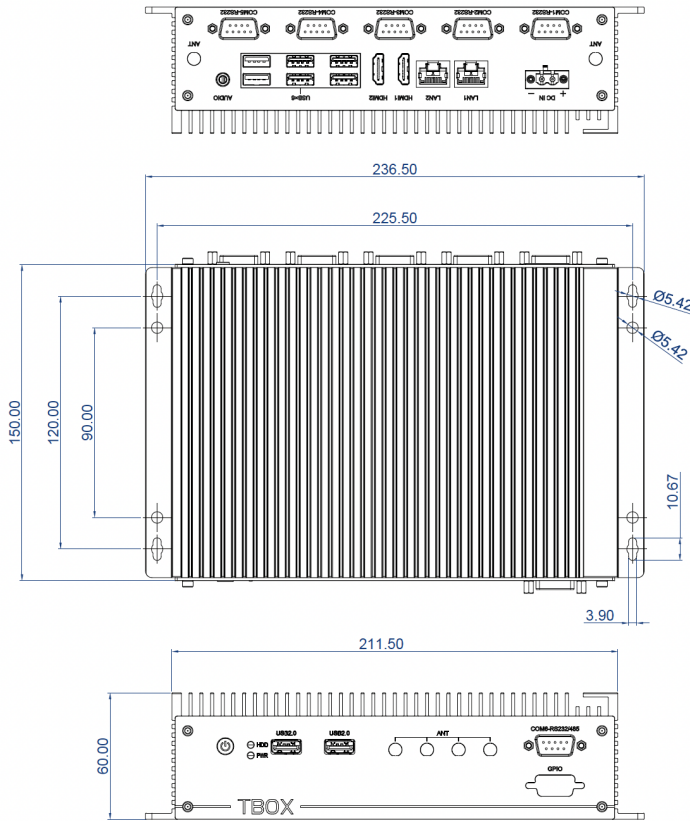
DIMENSIONAL DRAWING:TBOX-2EXX/2TXX
