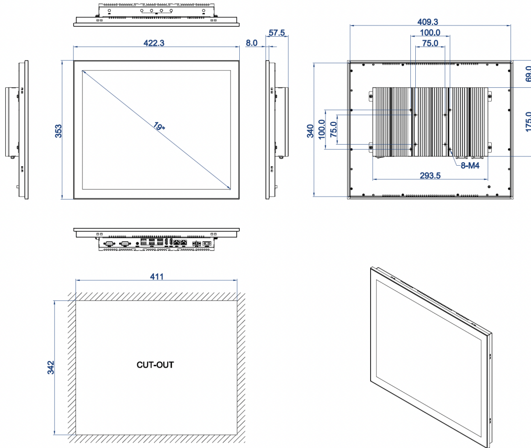
DIMENSIONAL DRAWING:TPC-DCS190E/T
