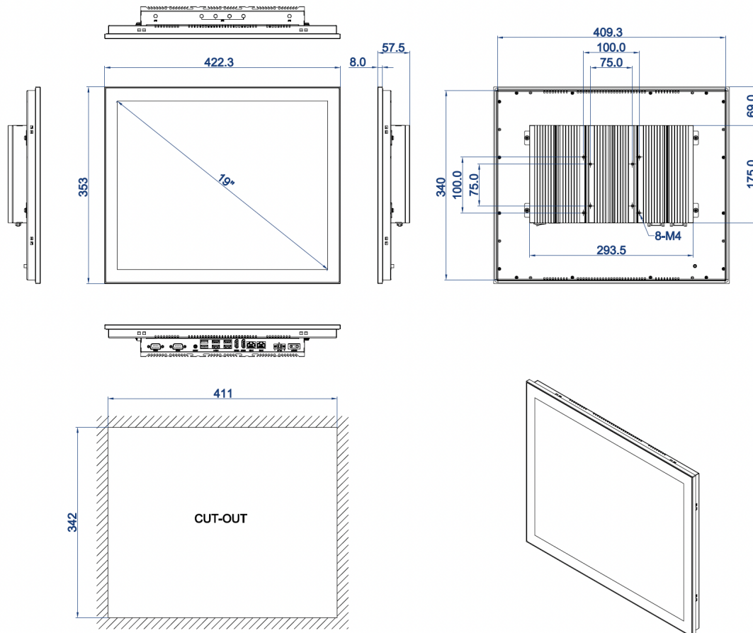
DIMENSIONAL DRAWING:TPC-DCS190E/T
