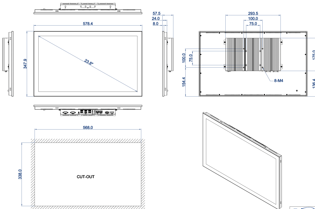
DIMENSIONAL DRAWING:TPC-DCS238E/T
