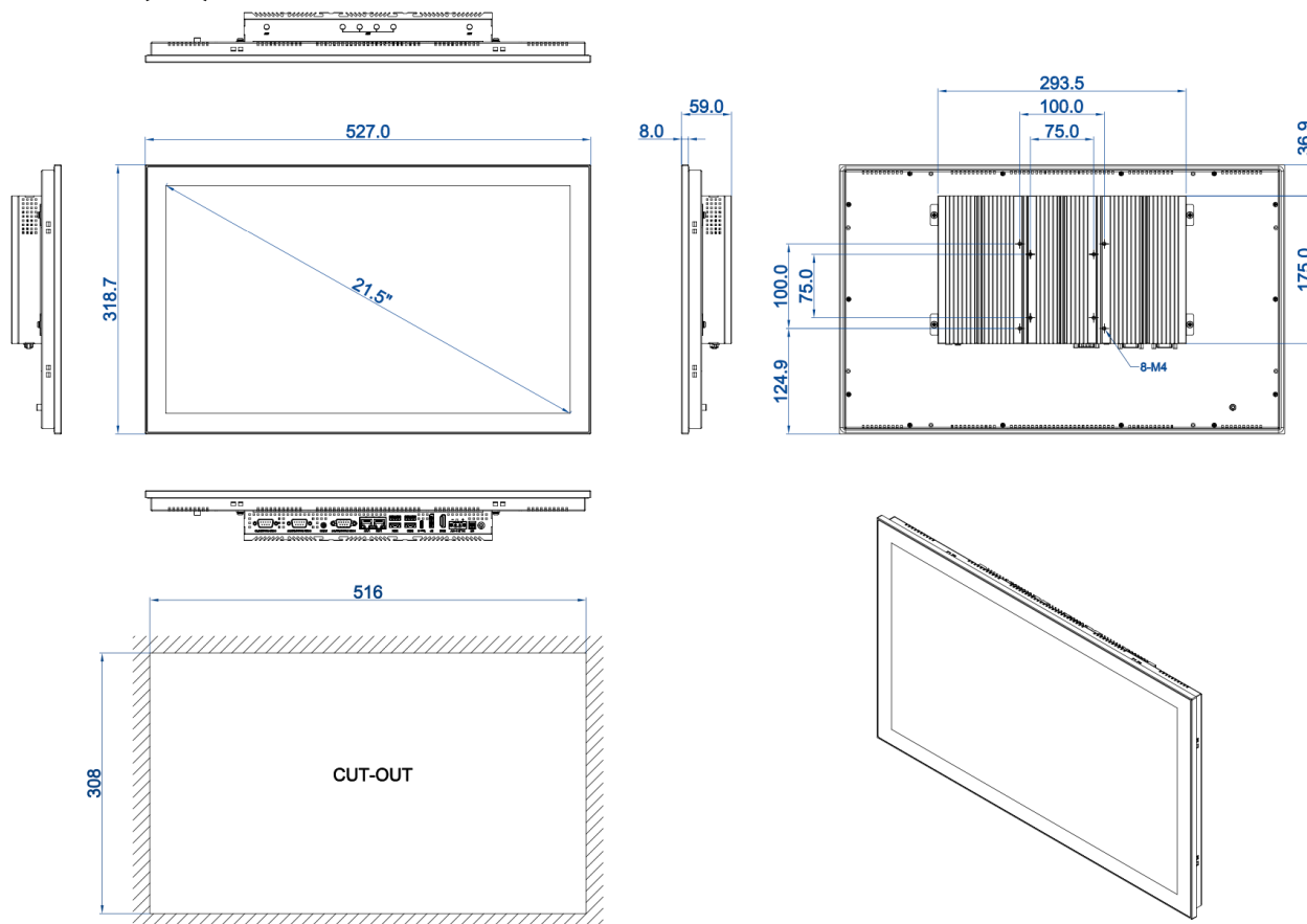
DIMENSIONAL DRAWING:TPC-DCT215D
