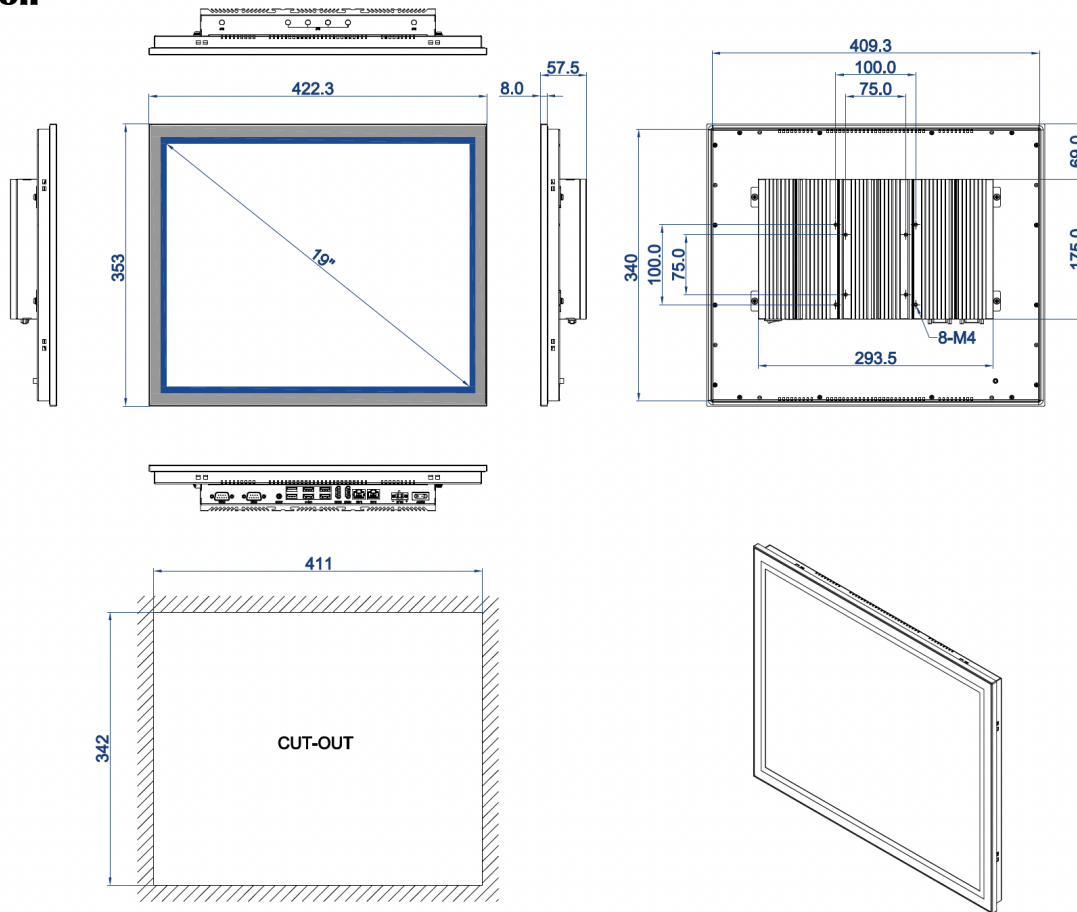
DIMENSIONAL DRAWING:TPC-DRS190ET
