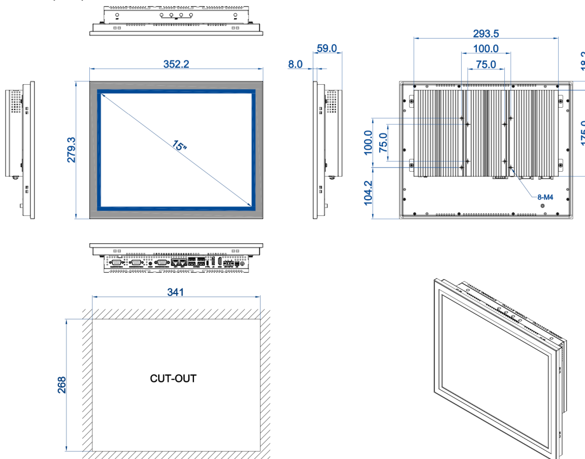
DIMENSIONAL DRAWING:TPC-DRT150D
