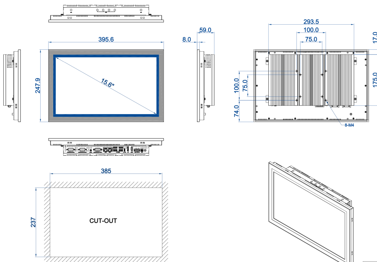
DIMENSIONAL DRAWING:TPC-DRT156D
