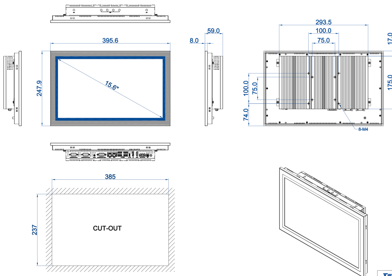
DIMENSIONAL DRAWING:TPC-DRT156D
