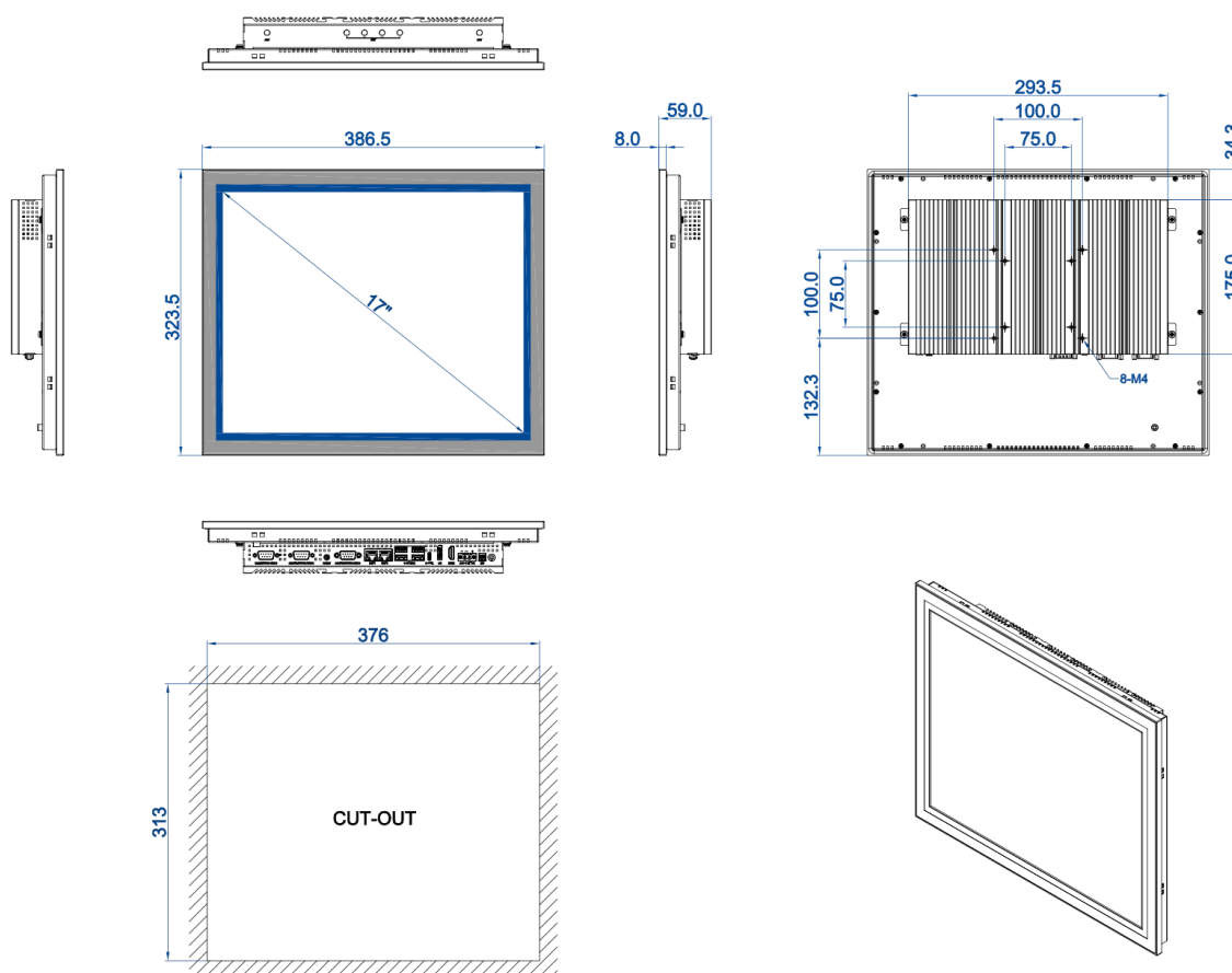
DIMENSIONAL DRAWING:TPC-DRT170D
