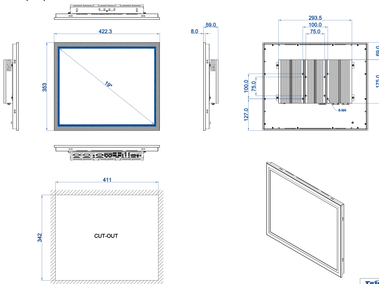
DIMENSIONAL DRAWING:TPC-DRT190D
