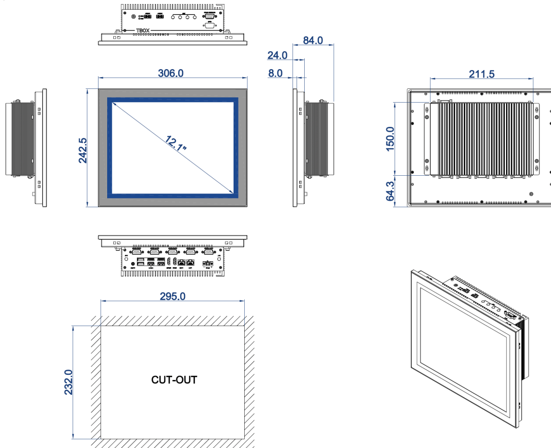
DIMENSIONAL DRAWING:TPC-PRS121E/T
