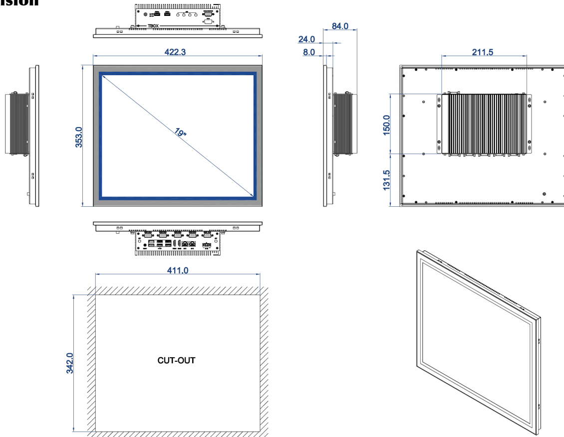
DIMENSIONAL DRAWING:TPC-PRS190E/T
