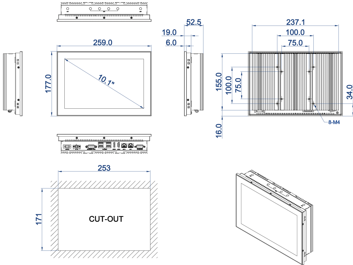
DIMENSIONAL DRAWING:TPC-DCS101A/W
