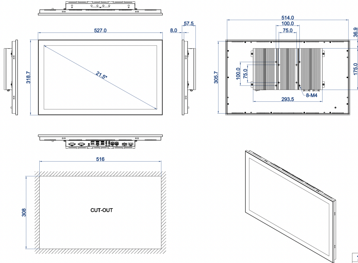
DIMENSIONAL DRAWING:TPC-DCS215E/T
