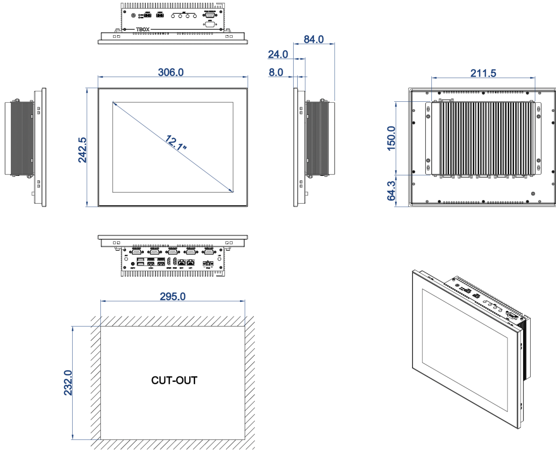
DIMENSIONAL DRAWING:TPC-PCS121E/T
