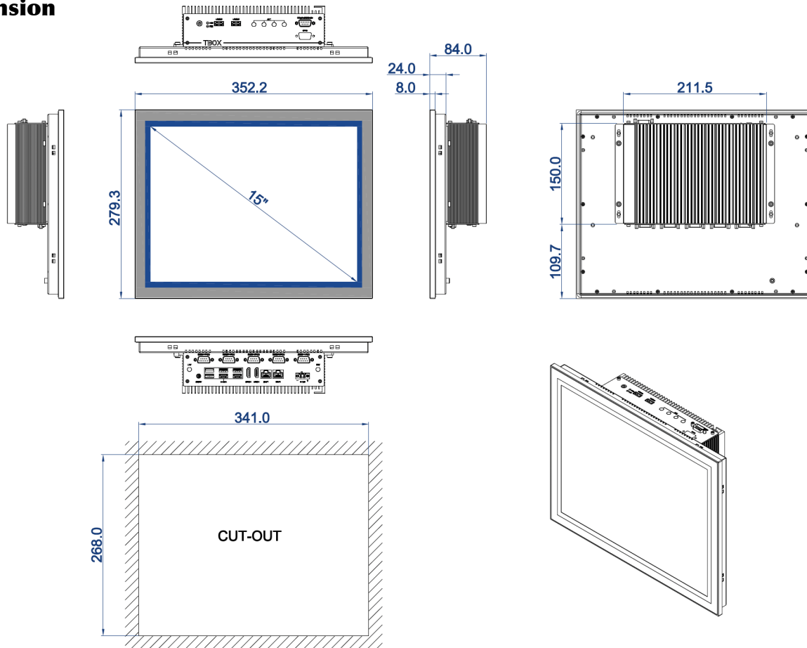
DIMENSIONAL DRAWING:TPC-PRS150E/T
