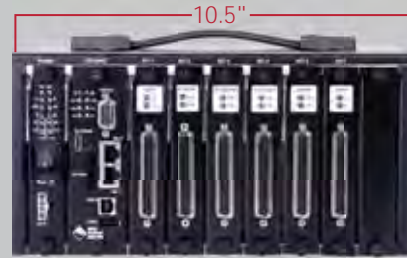
DNR-6-1G (HALF RACKtangle) 160,000 hours
